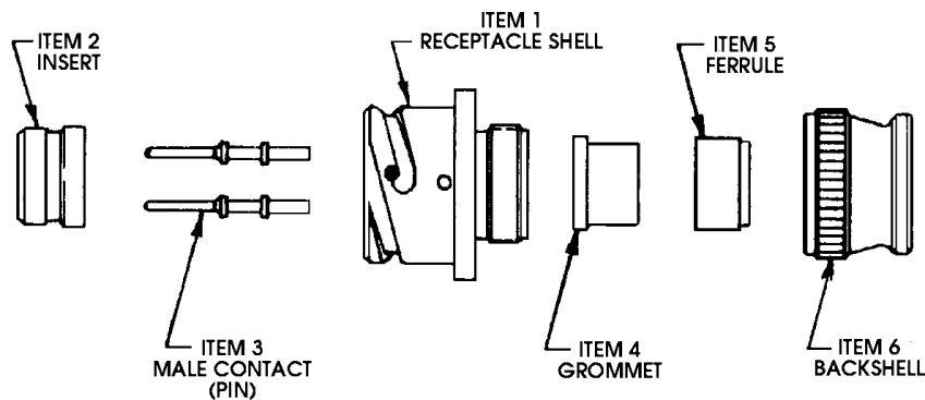
Figure 2. Exploded view of a typical "Receptacle" connector
