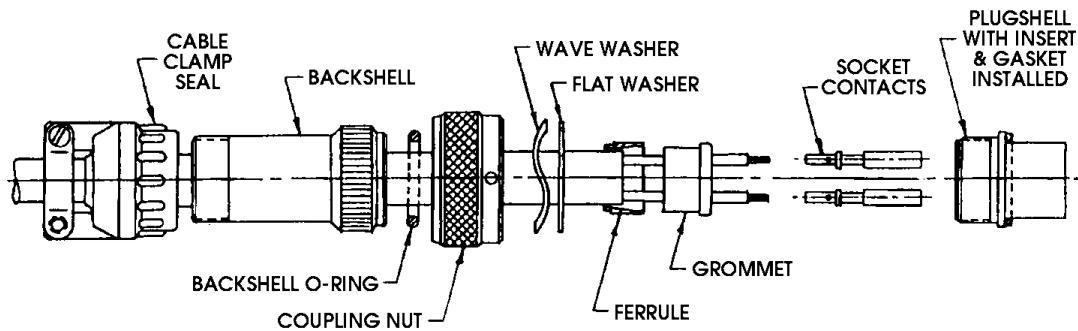
Figure 6. Jacketed Cable Connector Assembly Sequence
