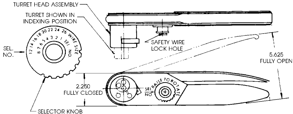
Figure 15 Crimp Tool M22520/1-01
