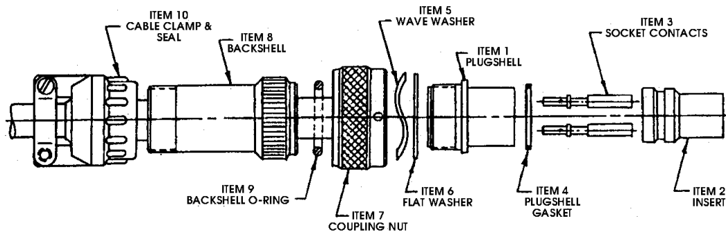
Figure 1. Exploded view of a typical "Plug" connector
